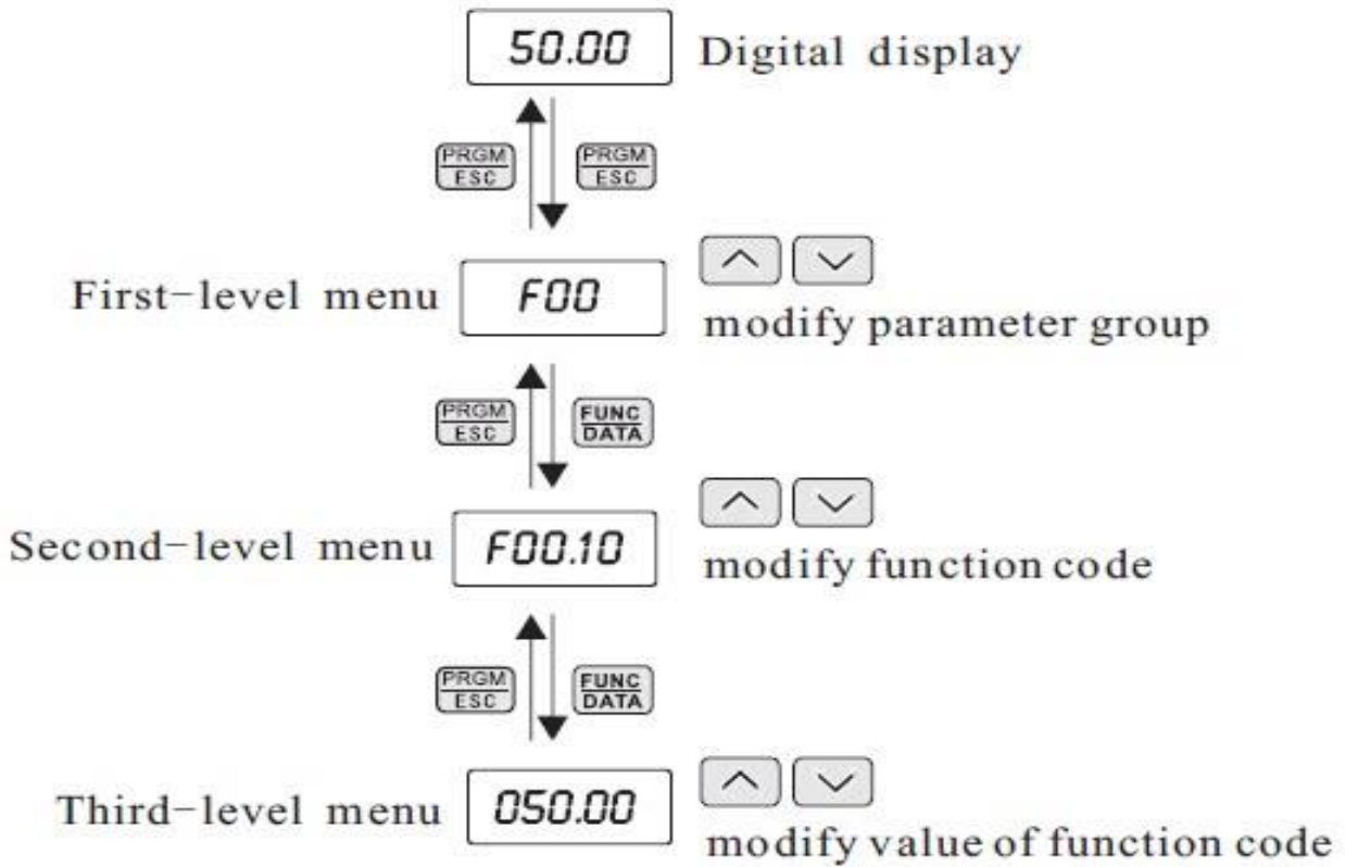
Operation flow chart of three-level menu
